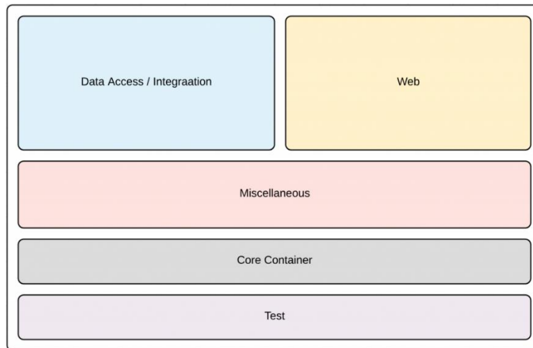
Figure 7: Spring Architecture
